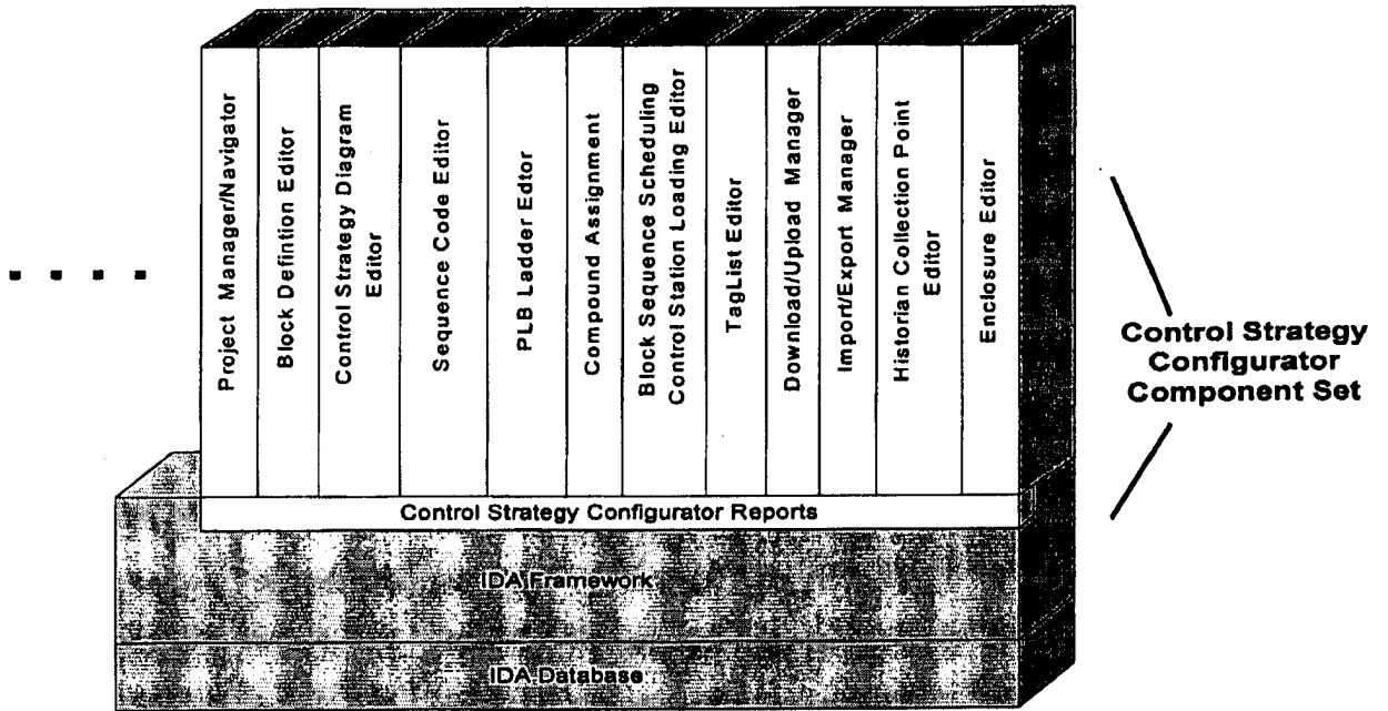
Figure 3 - Control Strategy Configurator Components
